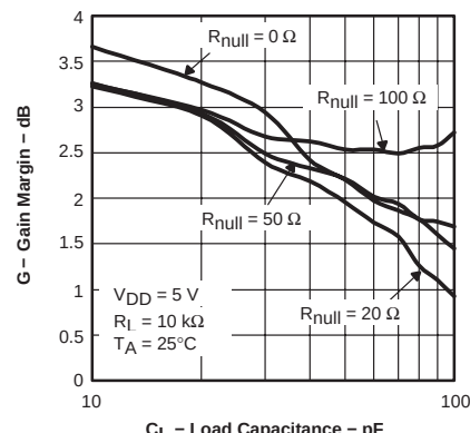
GAIN MARGIN VS LOAD CAPACITANCE
