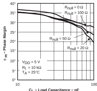
PHASE MARGIN VS LOAD CAPACITANCE
